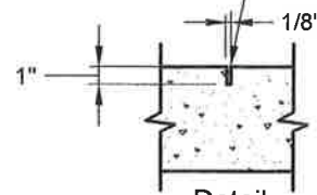
Detail Weakened Plane Joint
