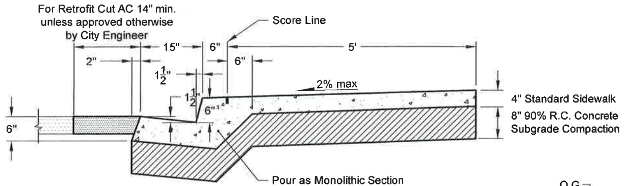
Curb, Gutter, & Sidewalk Section
