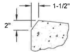
Chamfer Detail
