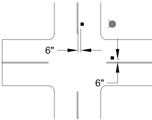
TWO LANE STREET AT INTERSECTION
