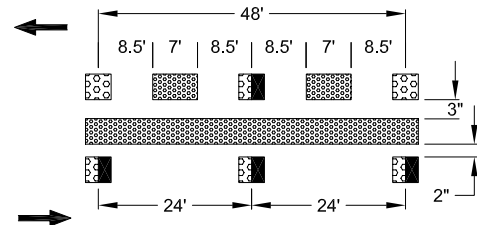
DETAIL 16
