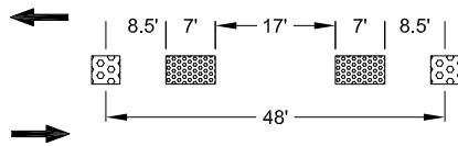
DETAIL 2
