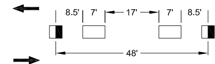
DETAIL 9
